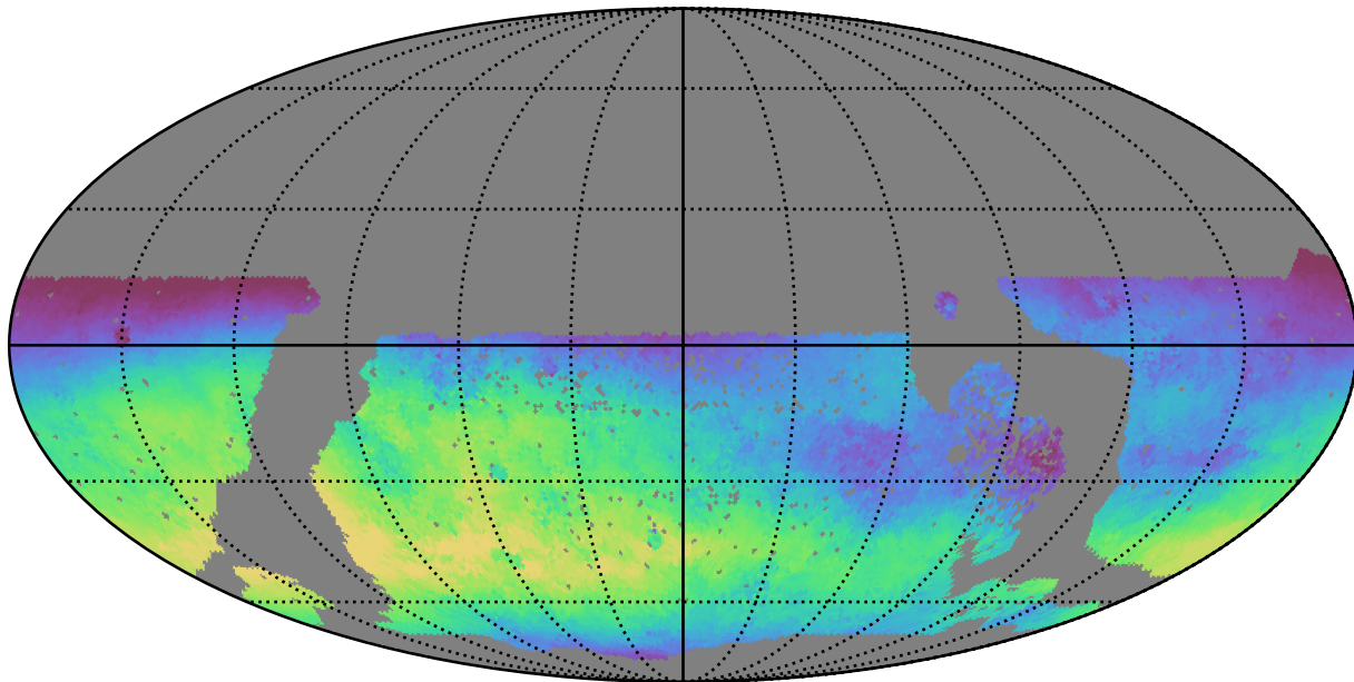
roman_v3.3_10yrs WFD u band: Median skyBrightness
