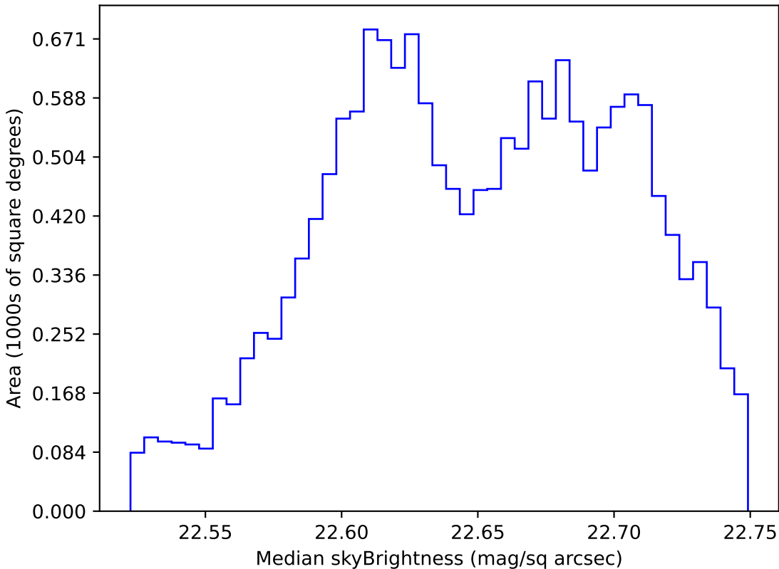
roman_v3.3_10yrs WFD u band: Median skyBrightness
