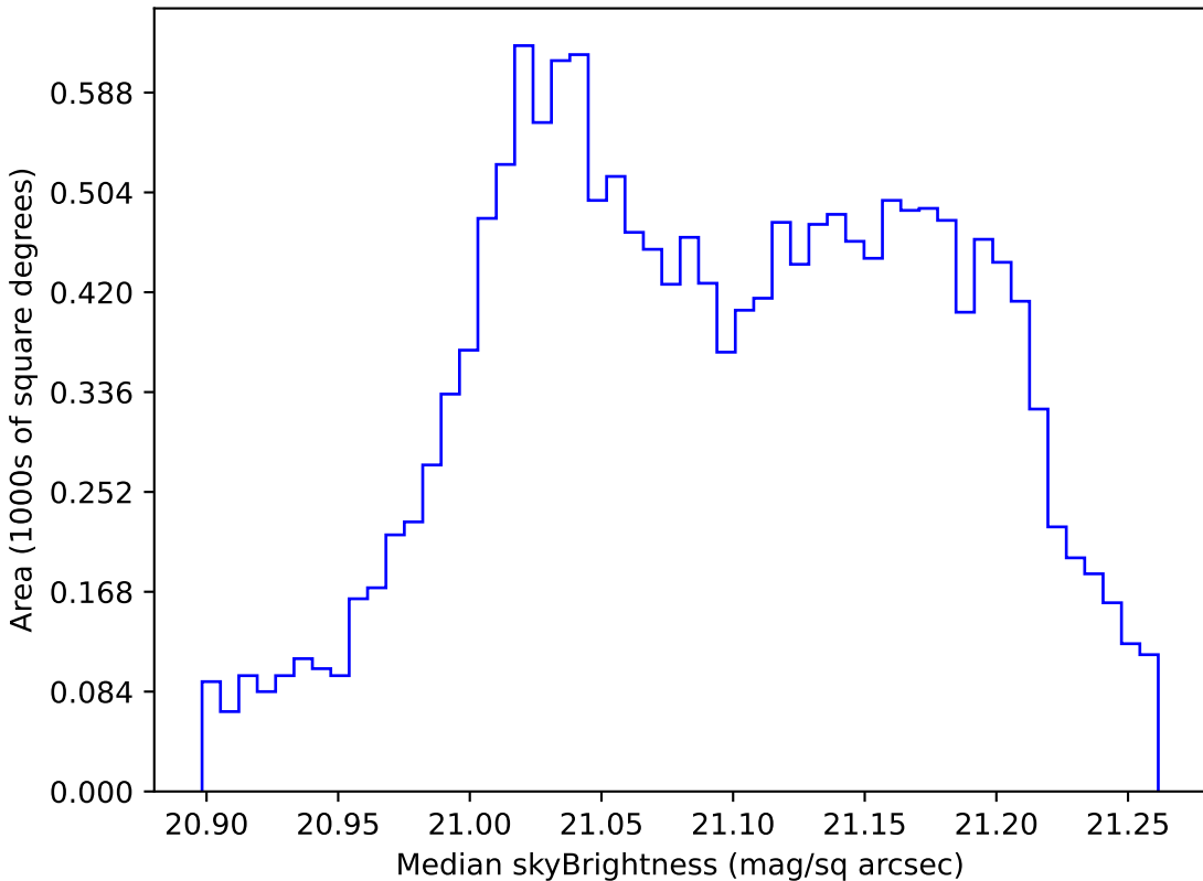
roman_v3.3_10yrs WFD r band: Median skyBrightness
