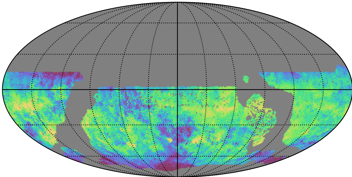
roman_v3.3_10yrs WFD i band: Median skyBrightness
