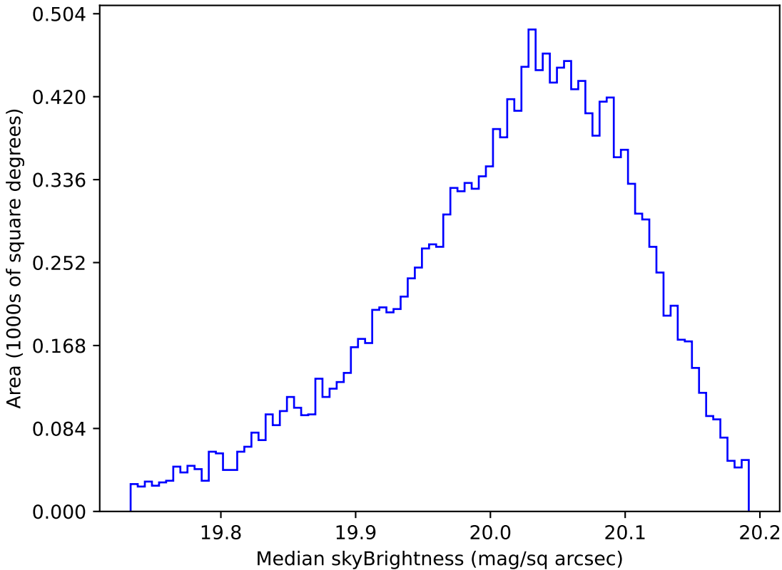
roman_v3.3_10yrs WFD i band: Median skyBrightness
