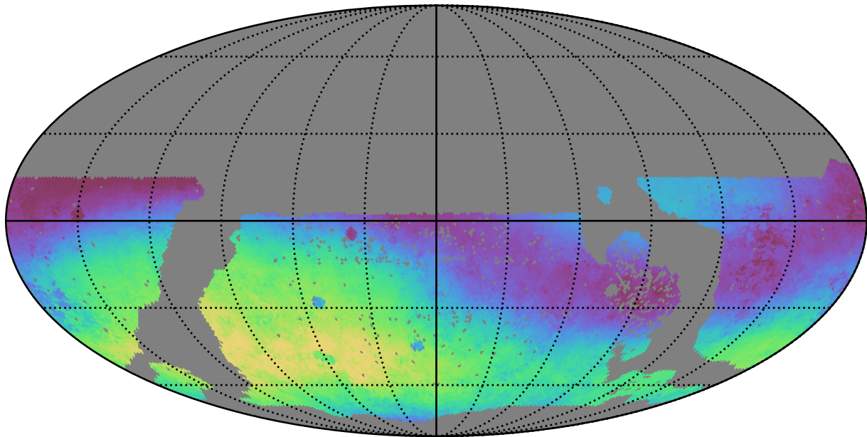
roman_v3.3_10yrs WFD g band: Median skyBrightness
