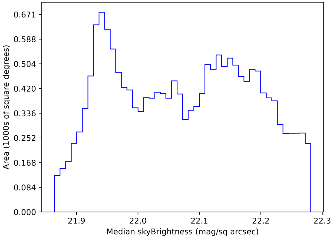
roman_v3.3_10yrs WFD g band: Median skyBrightness
