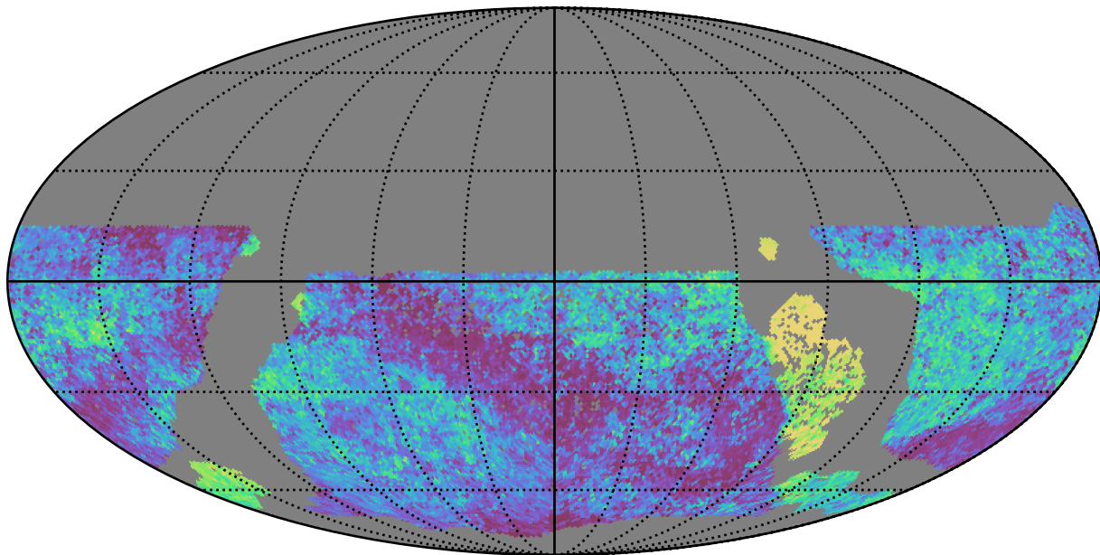
roman_v3.3_10yrs WFD all bands: Median skyBrightness
