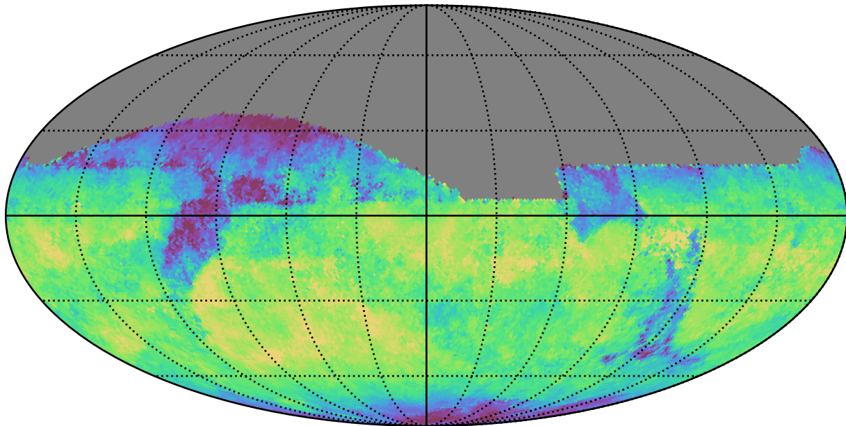
roman_v3.3_10yrs All sky z band: Median skyBrightness
