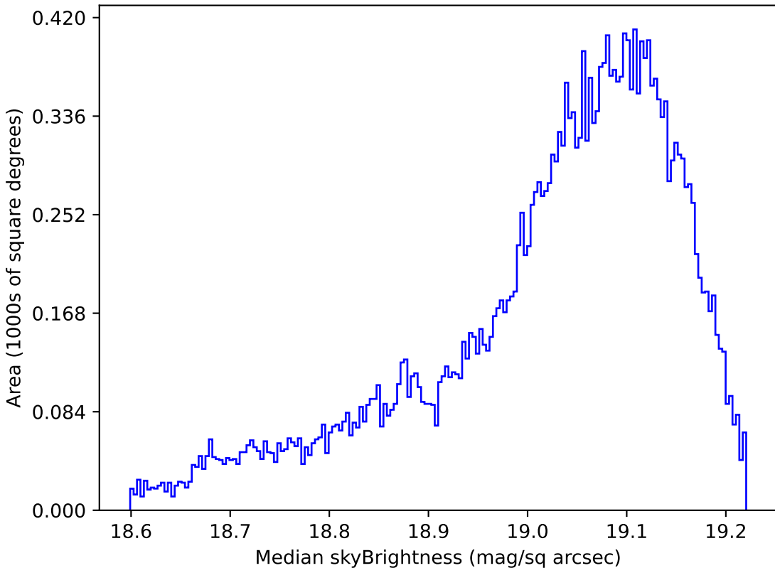
roman_v3.3_10yrs All sky z band: Median skyBrightness
