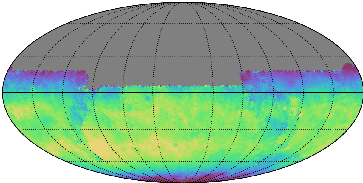
roman_v3.3_10yrs All sky y band: Median skyBrightness
