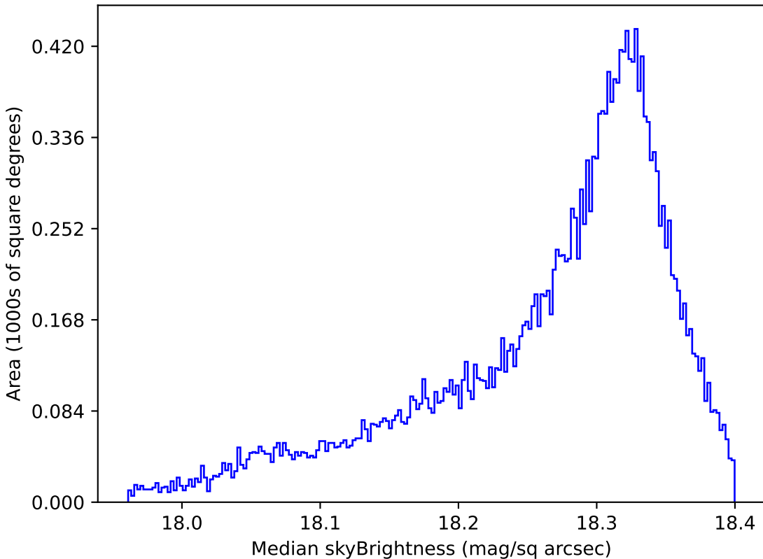
roman_v3.3_10yrs All sky y band: Median skyBrightness
