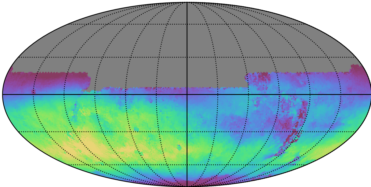
roman_v3.3_10yrs All sky u band: Median skyBrightness
