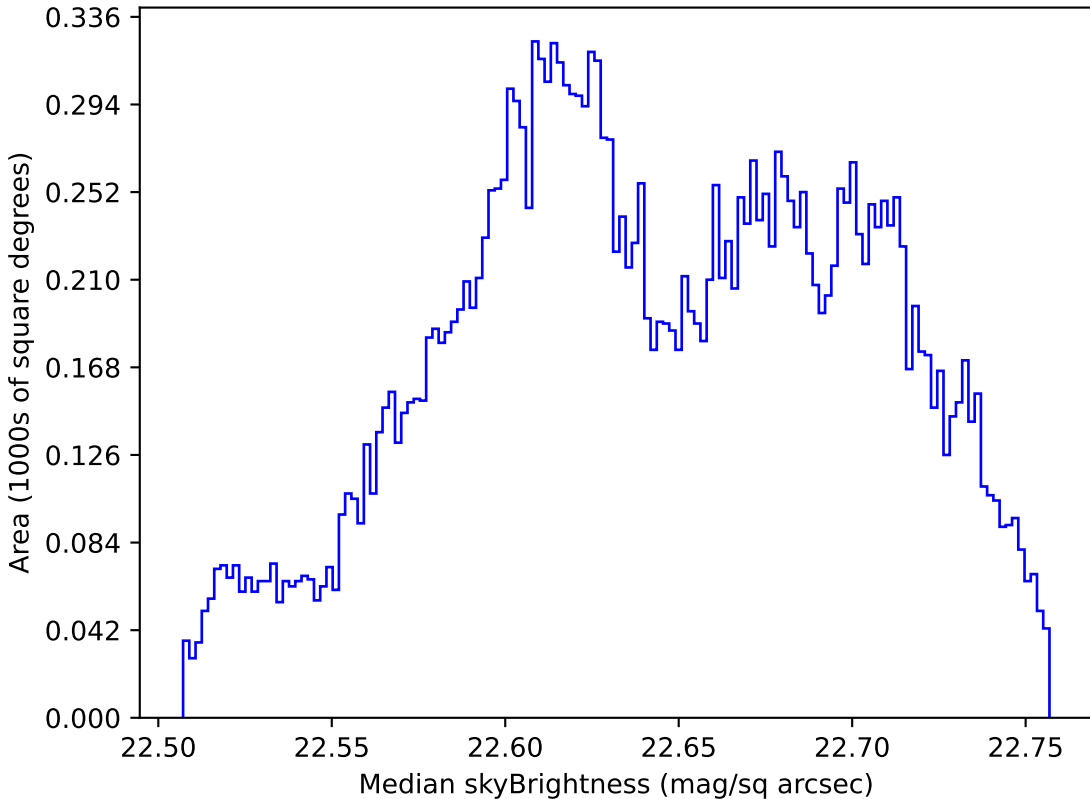
roman_v3.3_10yrs All sky u band: Median skyBrightness
