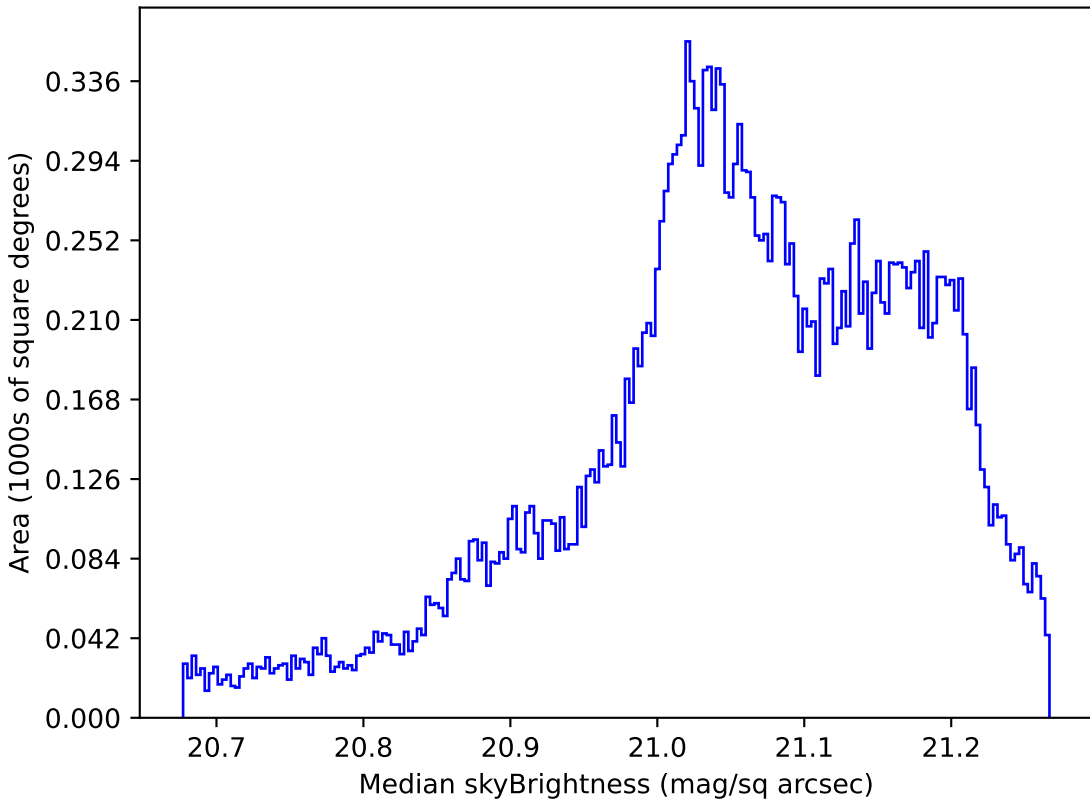
roman_v3.3_10yrs All sky r band: Median skyBrightness
