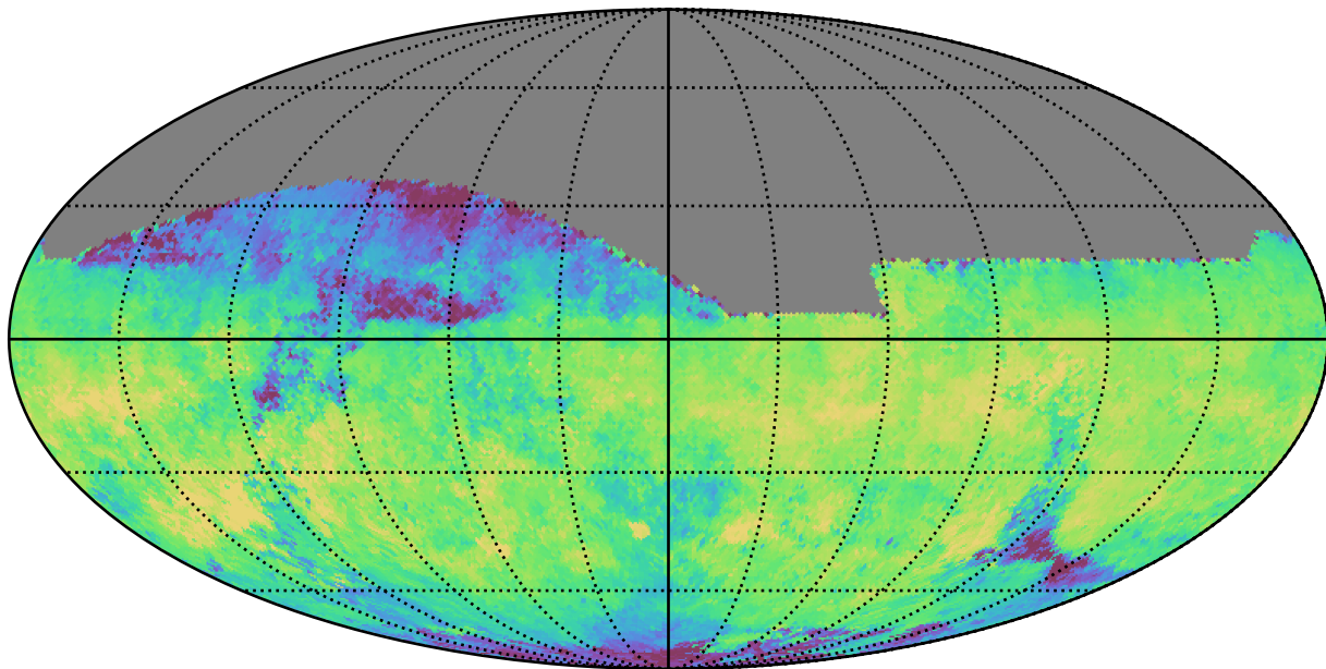
roman_v3.3_10yrs All sky i band: Median skyBrightness
