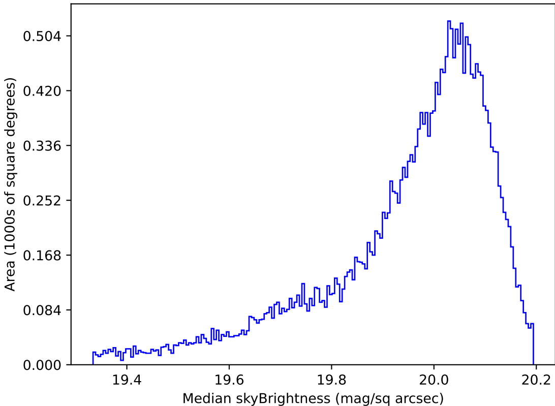
roman_v3.3_10yrs All sky i band: Median skyBrightness
