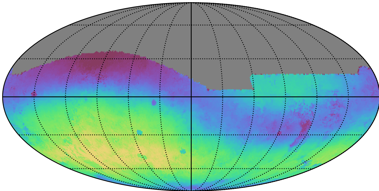
roman_v3.3_10yrs All sky g band: Median skyBrightness
