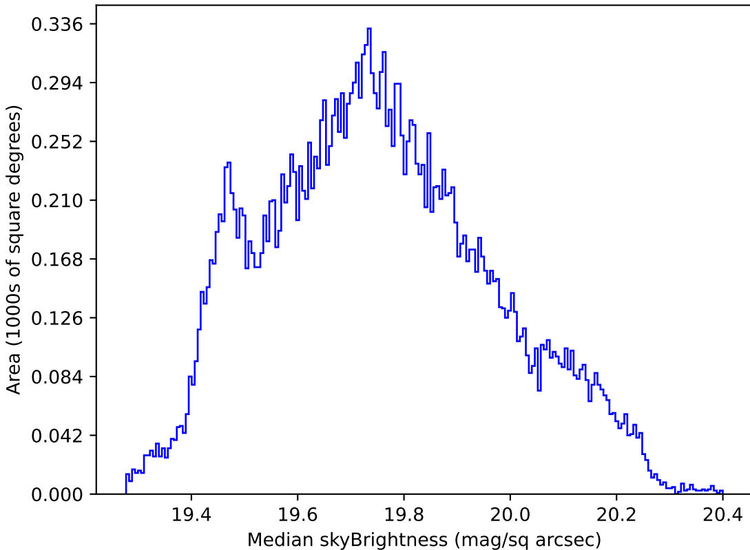
roman_v3.3_10yrs All sky all bands: Median skyBrightness
