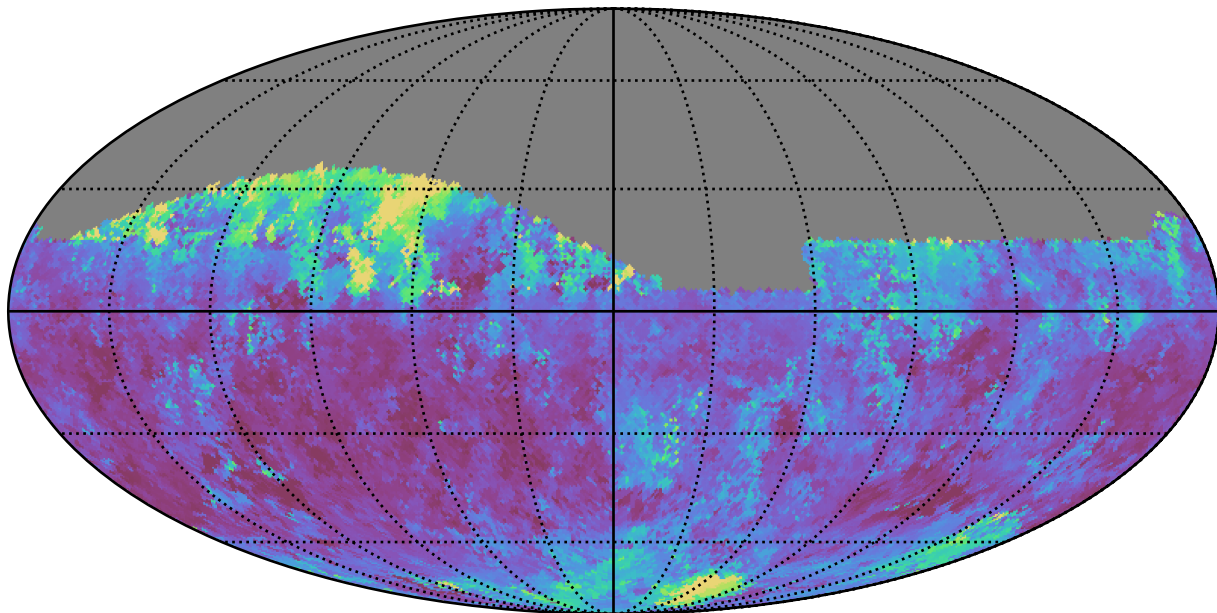
roman_v3.3_10yrs Yr 1 z band: Median seeingGeom
