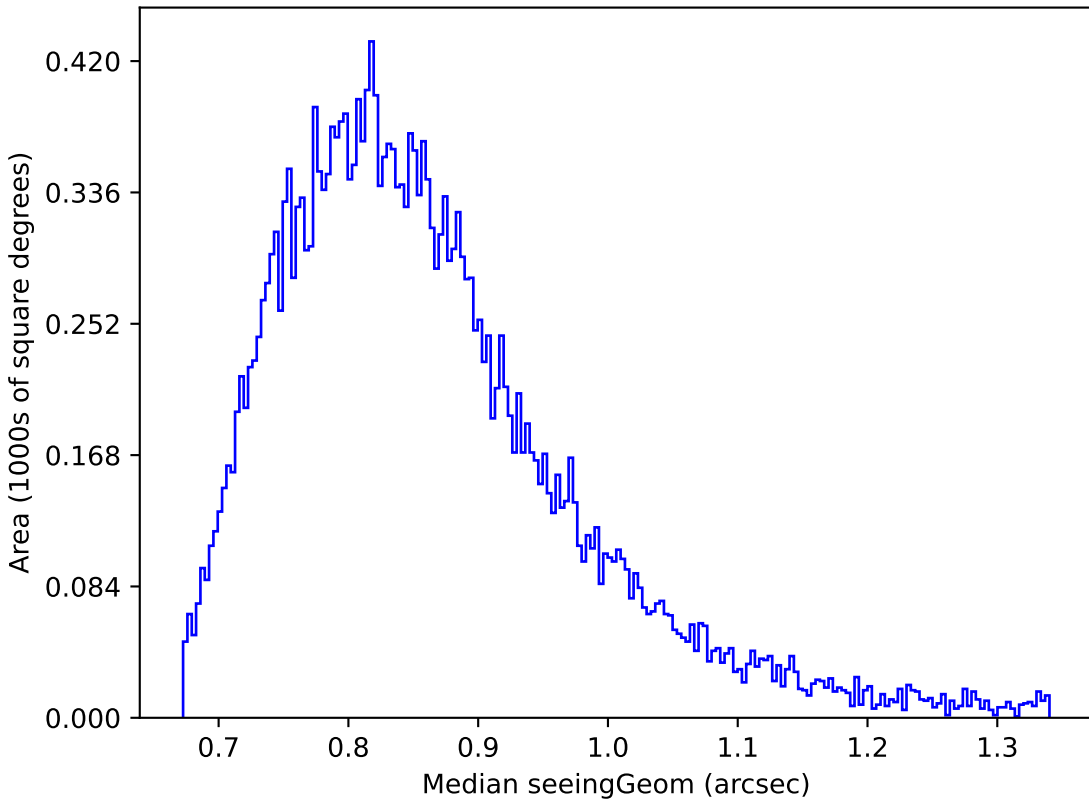
roman_v3.3_10yrs Yr 1 z band: Median seeingGeom
