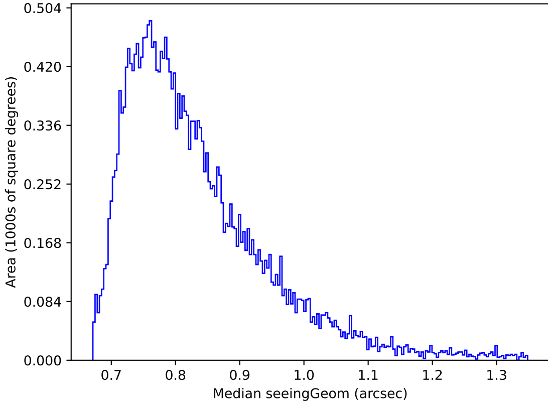
roman_v3.3_10yrs Yr 1 i band: Median seeingGeom
