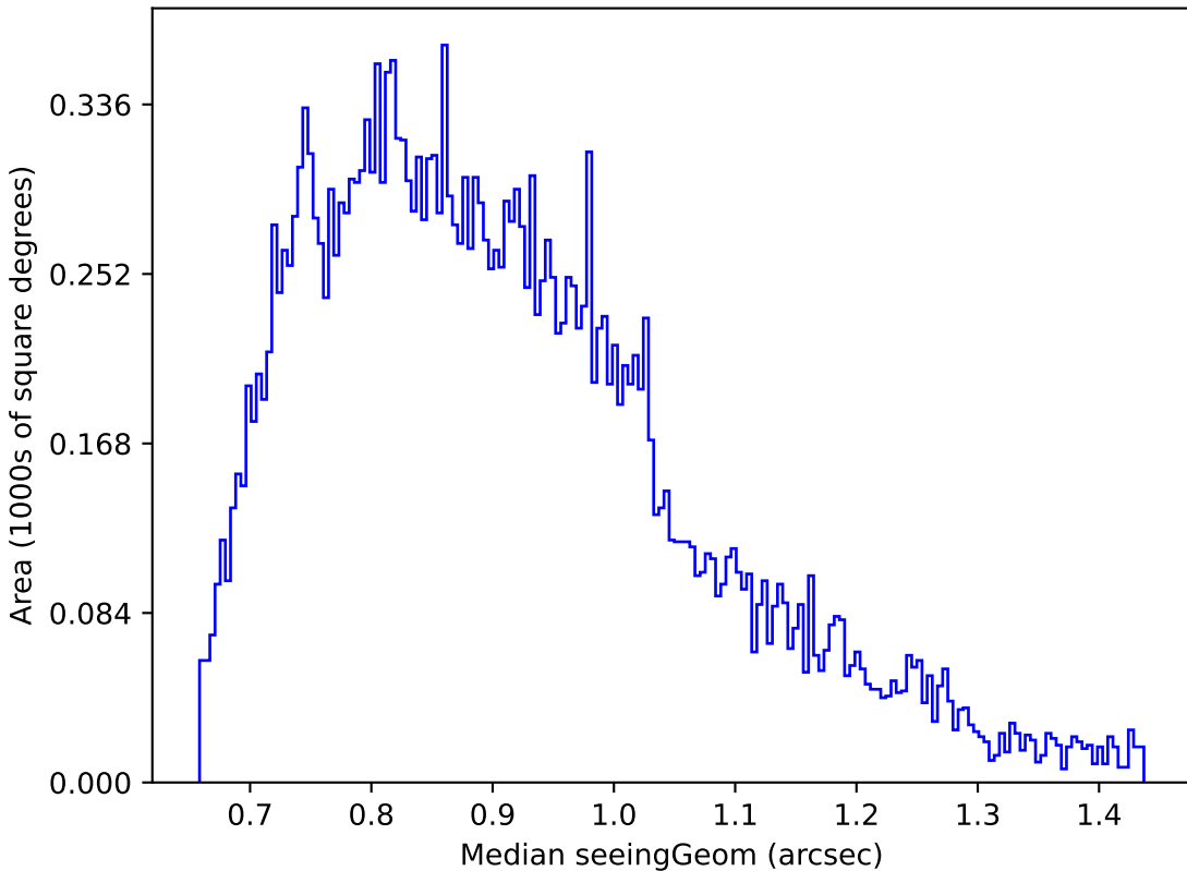
roman_v3.3_10yrs Yr 1 g band: Median seeingGeom
