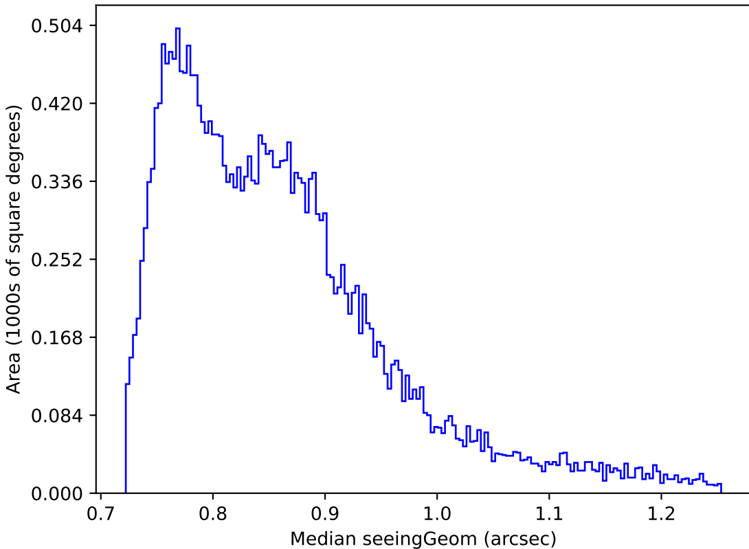
roman_v3.3_10yrs Yr 1 all bands: Median seeingGeom
