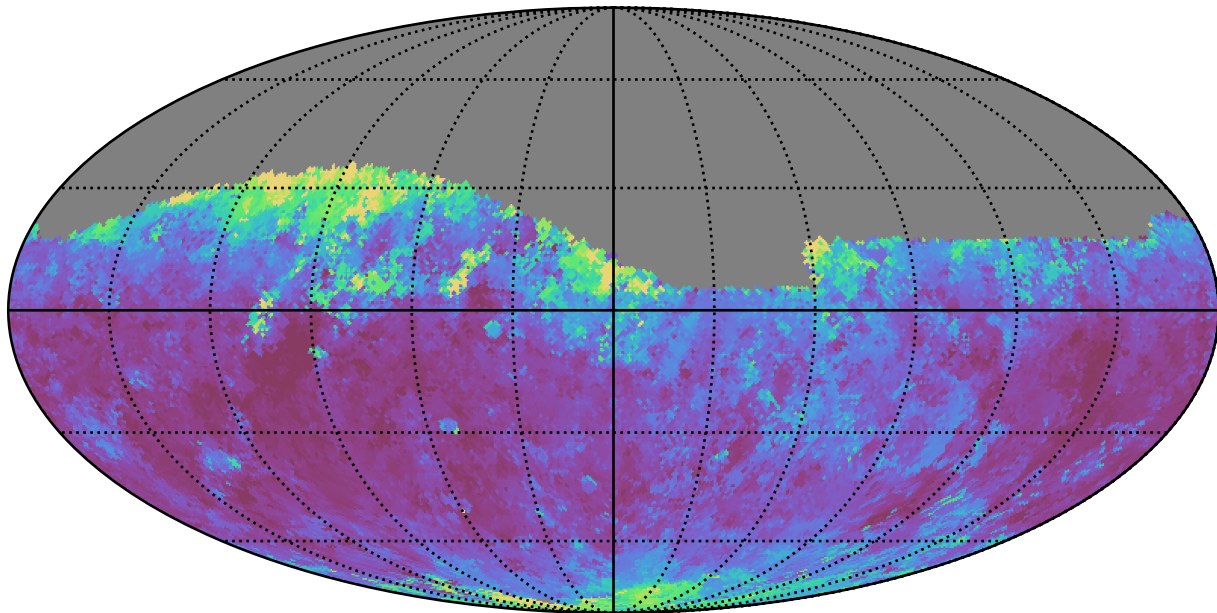
roman_v3.3_10yrs Yr 1 r band: Median seeingEff
