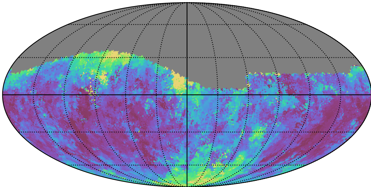
roman_v3.3_10yrs Yr 1 g band: Median seeingEff
