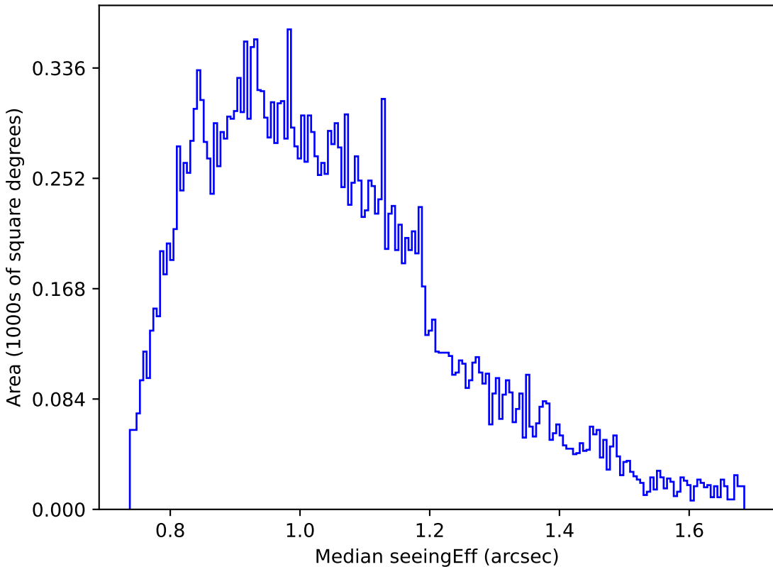
roman_v3.3_10yrs Yr 1 g band: Median seeingEff
