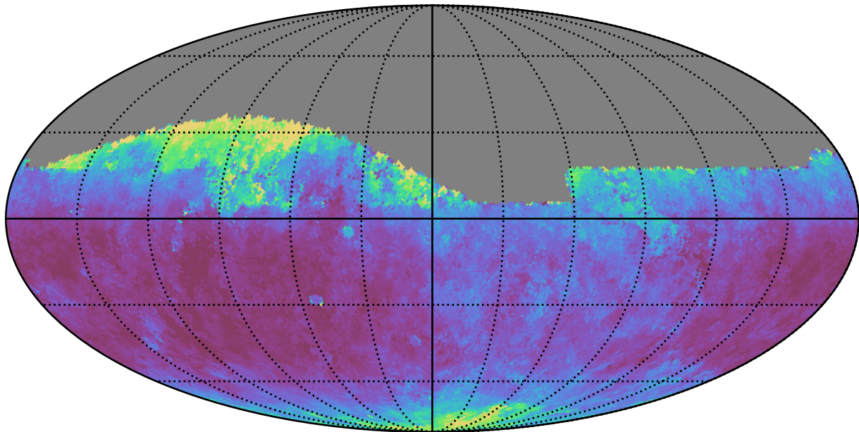
roman_v3.3_10yrs Yr 1 all bands: Median seeingEff
