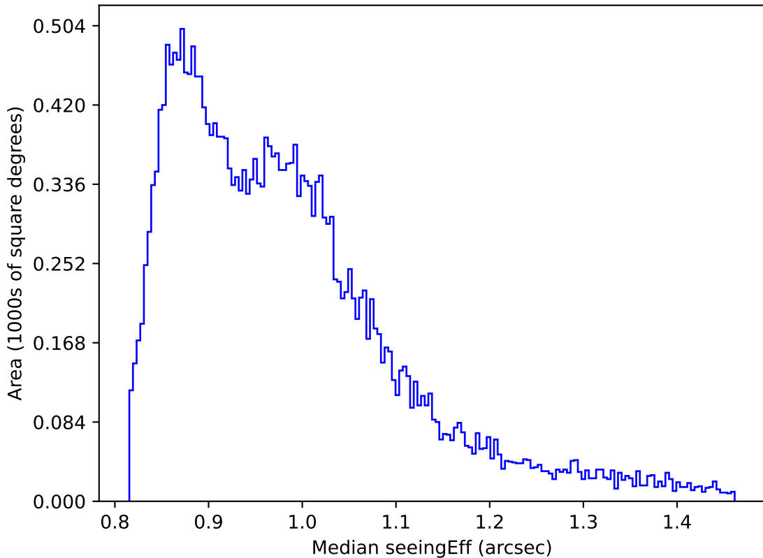
roman_v3.3_10yrs Yr 1 all bands: Median seeingEff
