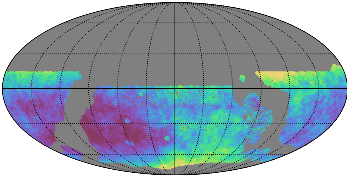
roman_v3.3_10yrs WFD z band: Median seeingEff
