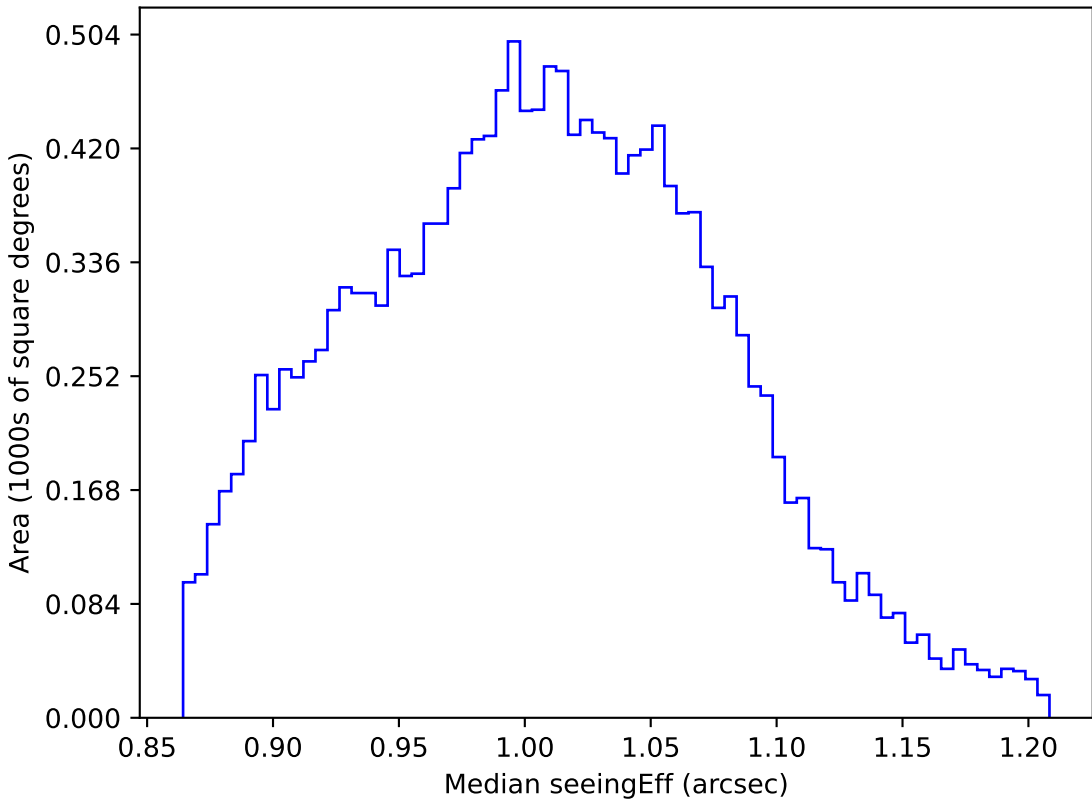
roman_v3.3_10yrs WFD z band: Median seeingEff
