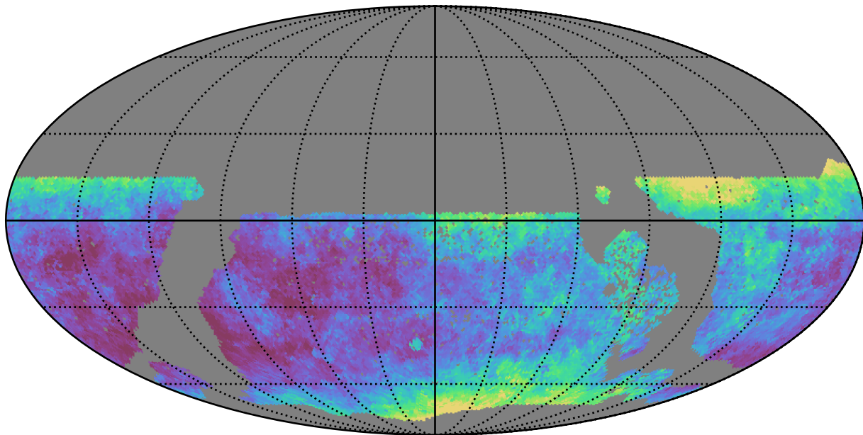
roman_v3.3_10yrs WFD y band: Median seeingEff
