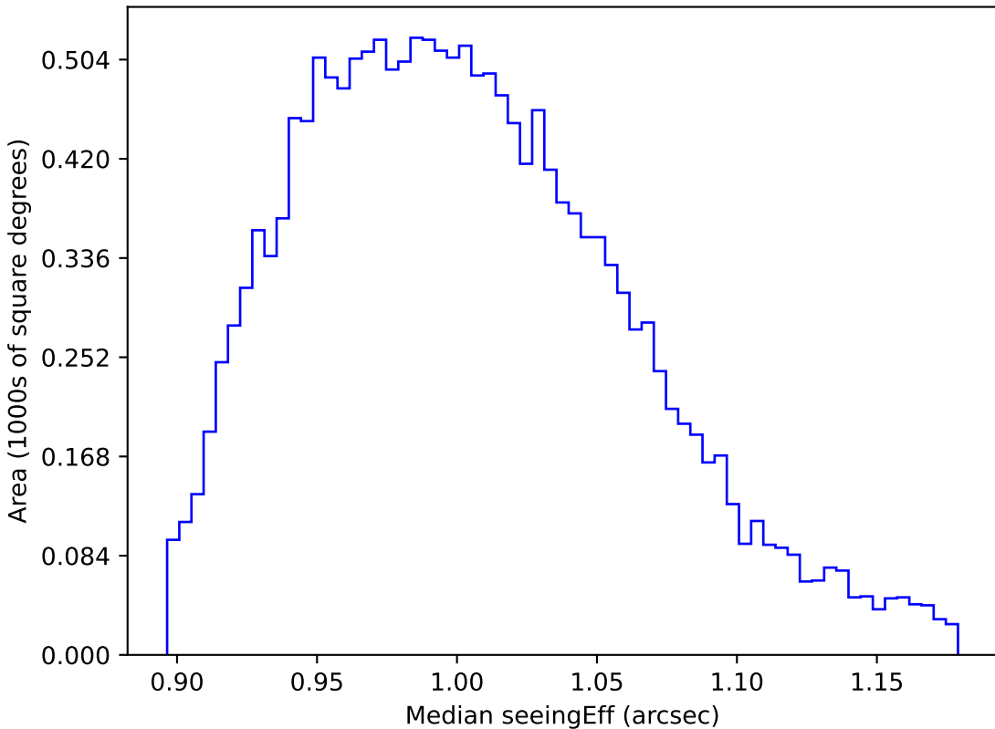
roman_v3.3_10yrs WFD y band: Median seeingEff
