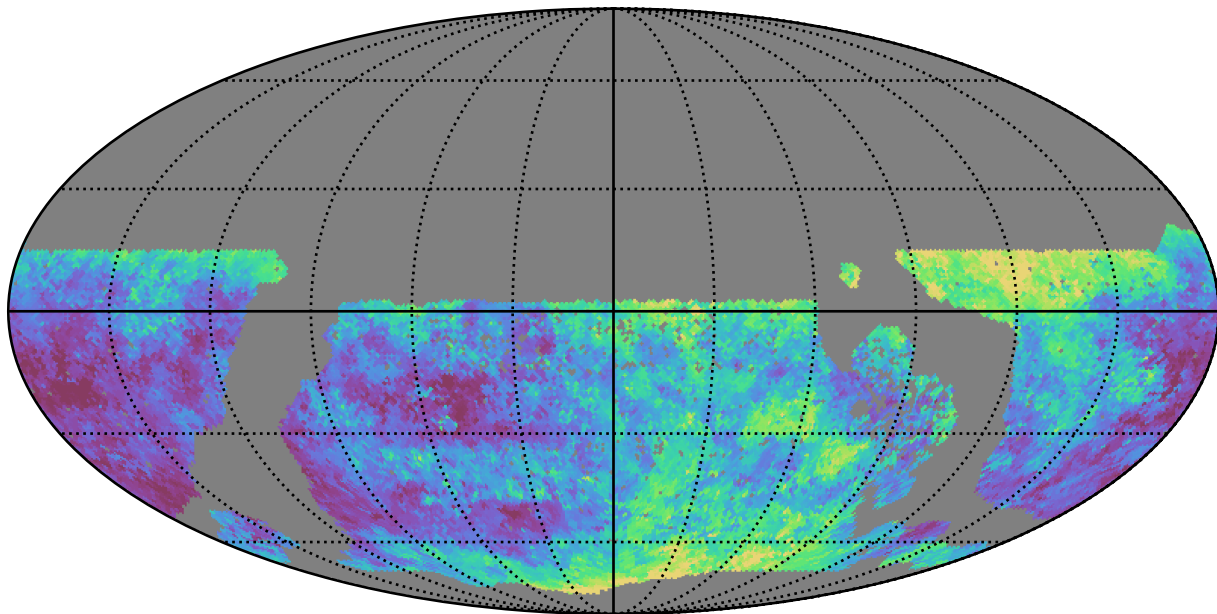
roman_v3.3_10yrs WFD u band: Median seeingEff
