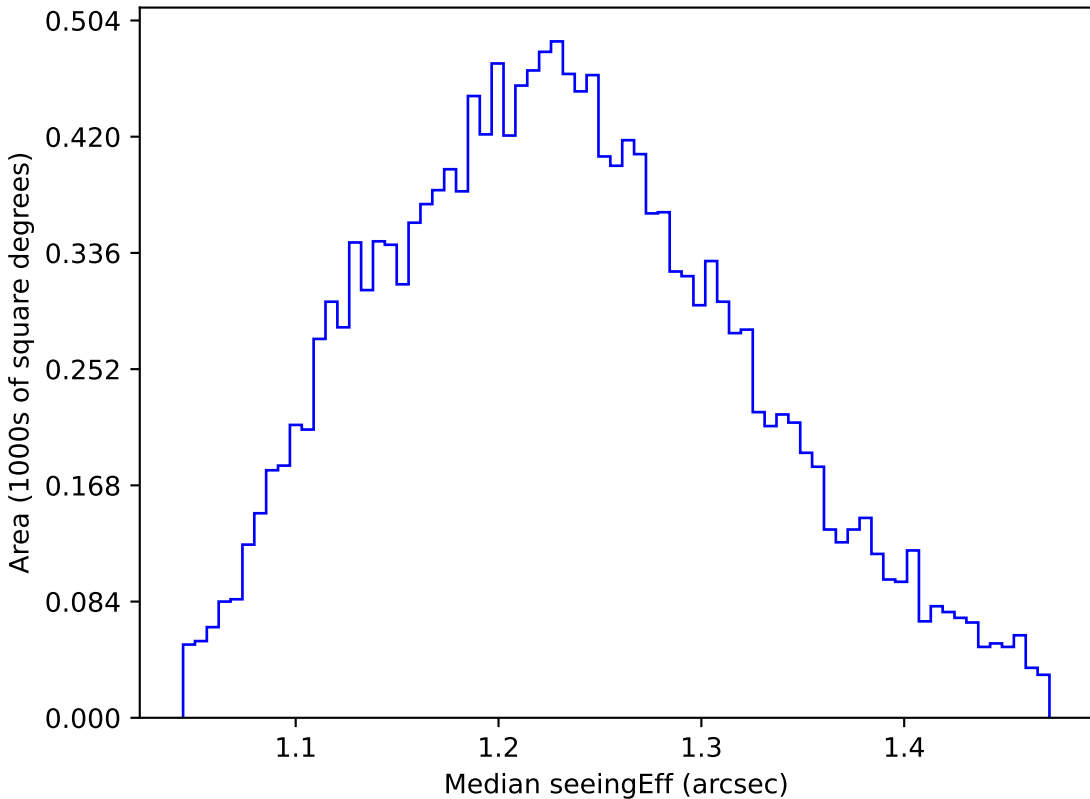
roman_v3.3_10yrs WFD u band: Median seeingEff
