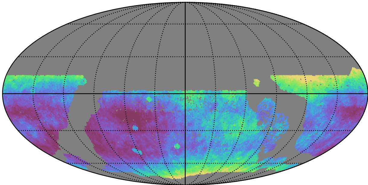
roman_v3.3_10yrs WFD r band: Median seeingEff
