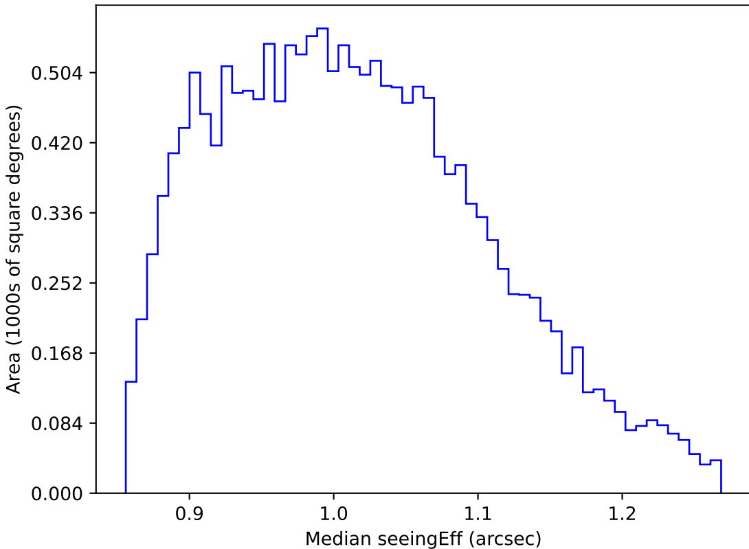
roman_v3.3_10yrs WFD r band: Median seeingEff
