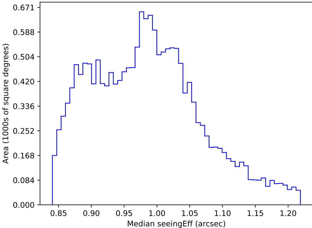
roman_v3.3_10yrs WFD i band: Median seeingEff
