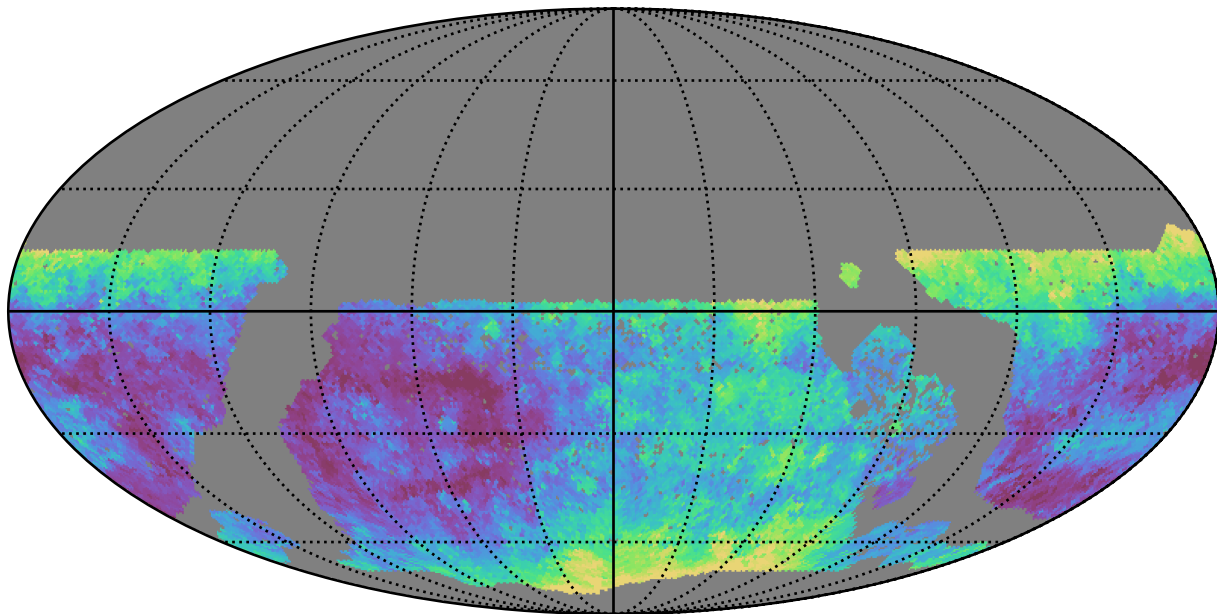
roman_v3.3_10yrs WFD g band: Median seeingEff
