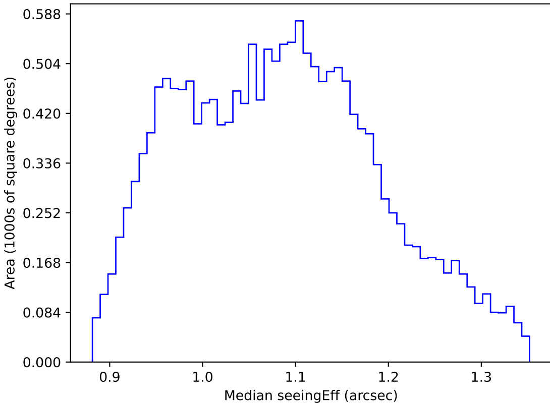
roman_v3.3_10yrs WFD g band: Median seeingEff
