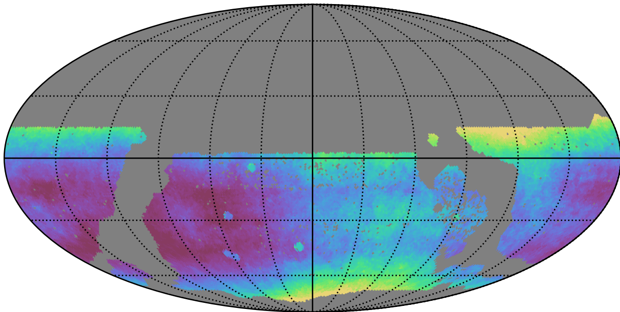
roman_v3.3_10yrs WFD all bands: Median seeingEff
