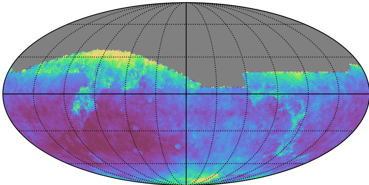
roman_v3.3_10yrs All sky z band: Median seeingEff
