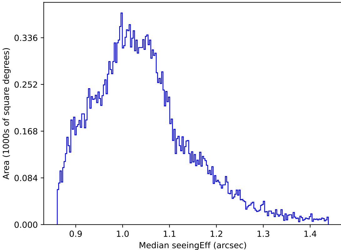
roman_v3.3_10yrs All sky z band: Median seeingEff
