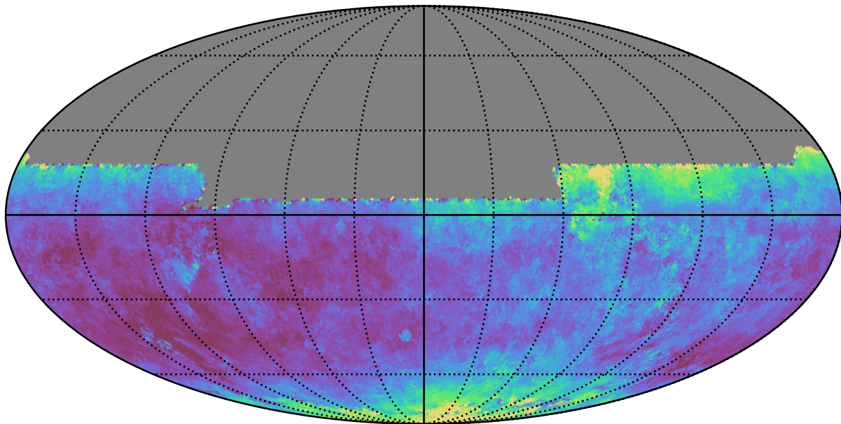
roman_v3.3_10yrs All sky y band: Median seeingEff
