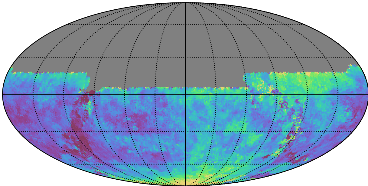
roman_v3.3_10yrs All sky u band: Median seeingEff
