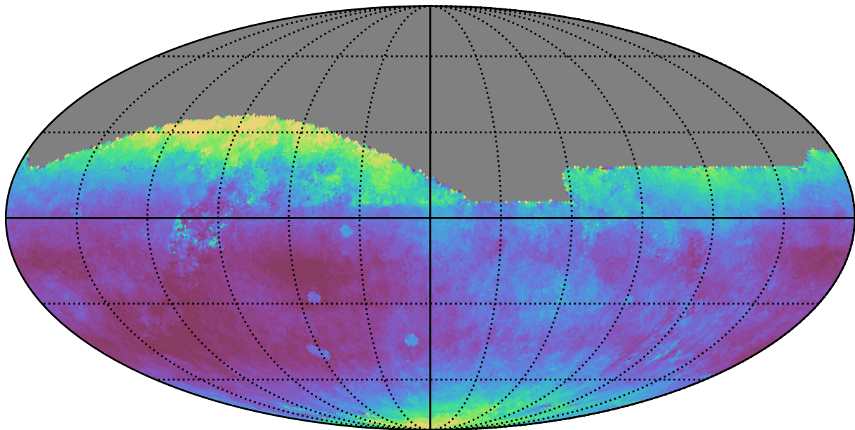
roman_v3.3_10yrs All sky r band: Median seeingEff
