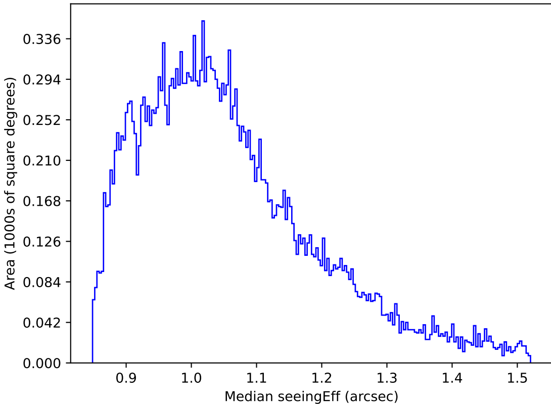
roman_v3.3_10yrs All sky r band: Median seeingEff
