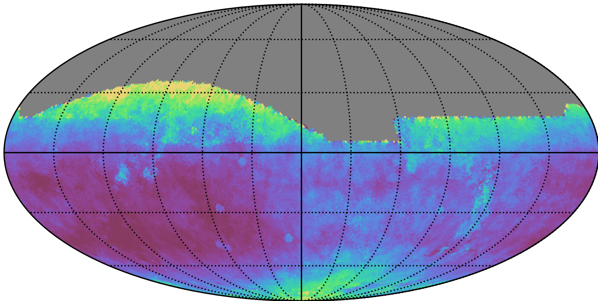
roman_v3.3_10yrs All sky i band: Median seeingEff
