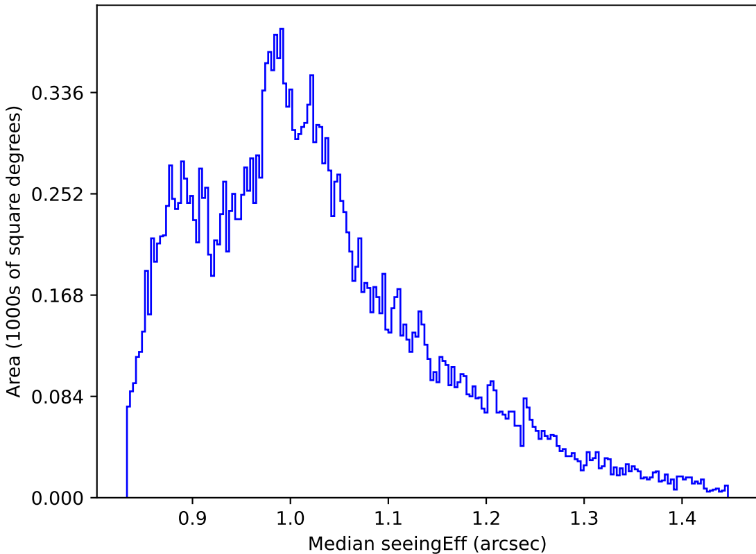
roman_v3.3_10yrs All sky i band: Median seeingEff
