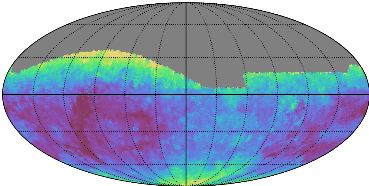
roman_v3.3_10yrs All sky g band: Median seeingEff
